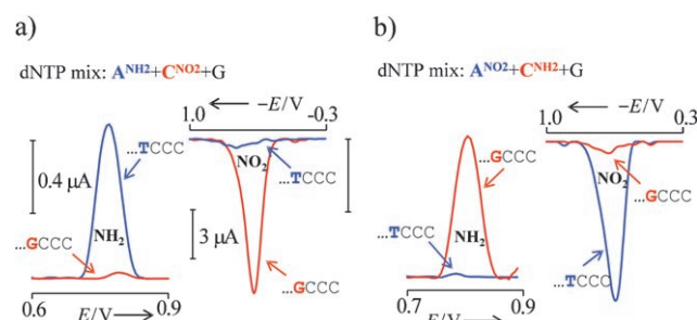
Figure 4. PEX probing of a SNP using nitro- and amino-labeled nucleotides. The PEX reactions were conducted with templates \text{temp}^A or \text{temp}^C (sequences complementary to the synthesized stretches shown) and a mixture of either a) \text{dA}^{\text{NO}_2}\text{TP} + \text{dC}^{\text{NH}_2}\text{TP} or b) \text{dA}^{\text{NH}_2}\text{TP} + \text{dC}^{\text{NO}_2}\text{TP} (complemented with unlabeled dGTP). Sections of voltammograms spanning the incorporated label signals are shown. Other details as in Figure 2.
