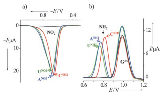
Figure 3. SWV responses of pex md16 products bearing a) nitrophenyl or b) aminophenyl labels synthesized using mixtures of labeled dNTPs (blue, dA NO 2 TP or dA NH 2 TP; green, dU NO 2 TP or dU NH 2 TP; red, dC NO 2 TP or dC NH 2 TP) with unlabeled dNTPs to complete the synthesized sequence (see Figure 1), and 5'-biotinylated templates. Black curves correspond to the unlabeled PEX product. The PEX reaction was catalyzed by Klenow polymerase. Prior to SWV measurements, the extended primer strands were isolated by a magnetoseparation procedure (see the Supporting Information). G ox : signal from the electro-oxidation of guanine.
