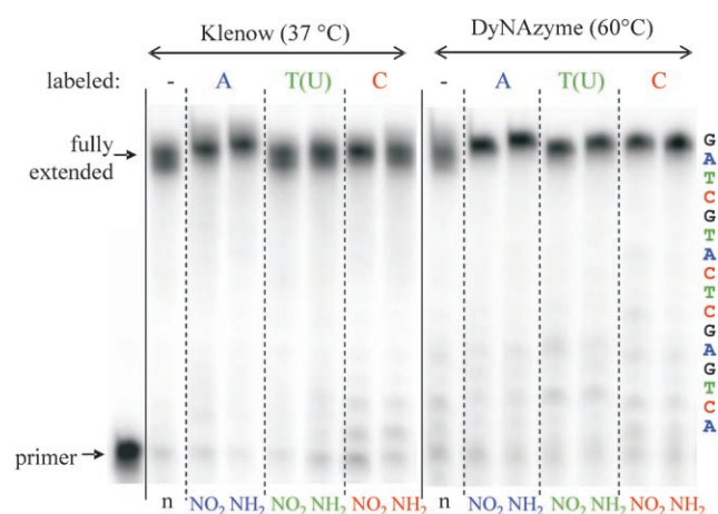
Figure 1. Denaturing PAGE analysis of PEX products synthesized on template temp md16 using dNTP mixes containing one of the nitrophenyl or aminophenyl dNTP conjugates (dA NH 2 TP, dA NO 2 TP, dU NH 2 TP, dU NO 2 TP, dC NH 2 TP, or dC NO 2 TP) complemented by the remaining three unmodified dNTPs.
