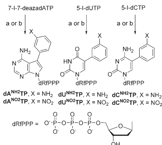
Scheme 1. Reagents and conditions: 3-aminophenylboronic acid (a) or 3-nitrophenylboronic acid (b) and Cs 2 CO 3 , Pd(OAc) 2 , P(C 6 H 4 -3-SO 3 Na) 3 , H 2 O/CH 3 CN (2:1).
