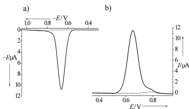
Figure 2. Square-wave voltammetry (SWV) signals resulting from a) nitro group reduction in dU NO 2 TP or b) amino group oxidation in dU NH 2 TP at a pyrolytic graphite electrode. Dotted curves correspond to unmodified dTTP. For more details, see the Supporting Information.
